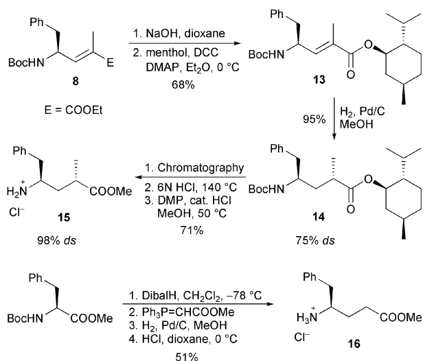
Scheme 3. Synthesis of Tup ( 15 ) and dTup ( 16 ).
