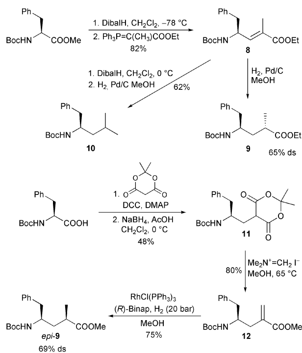
Scheme 2. Synthetic attempts directed towards Tup.
