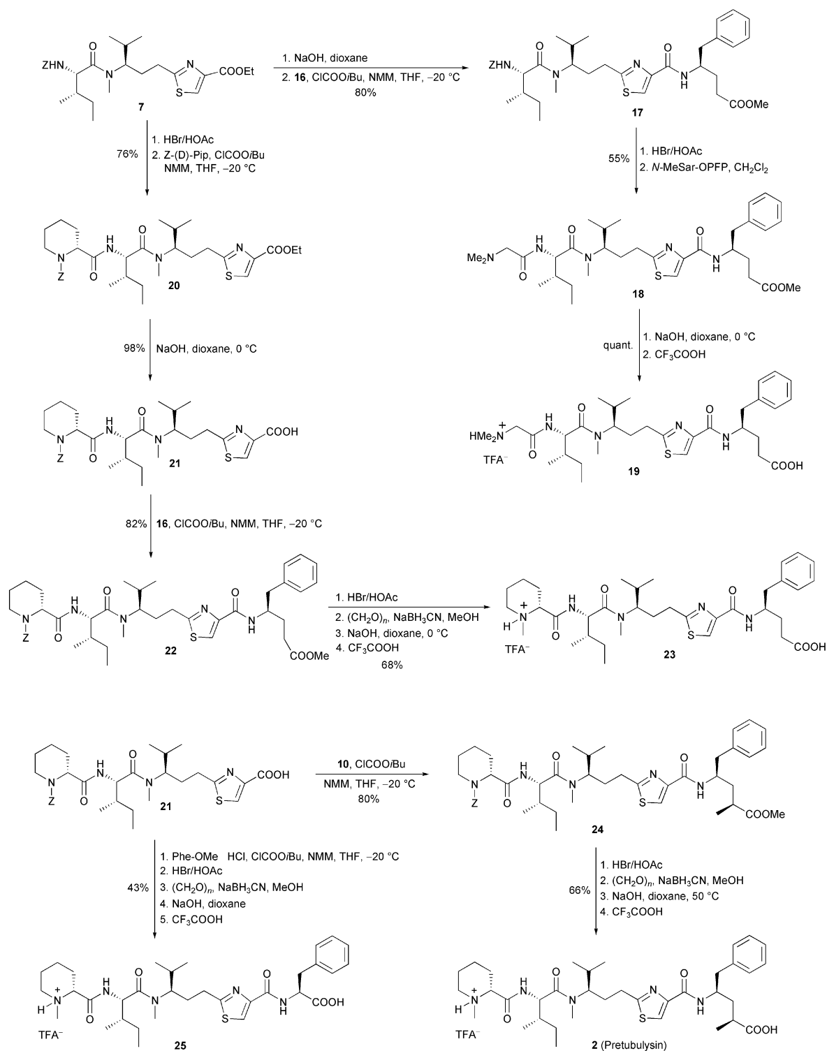
Scheme 4. Synthesis of pretubulylin and simplified derivatives.
