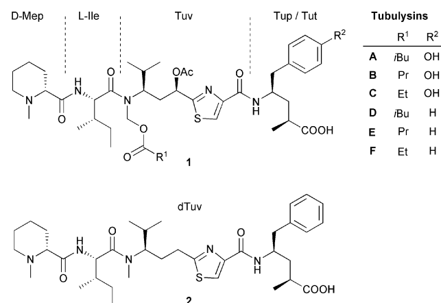
Figure 1. Selected tubulysins ( 1 ) and pretubulysin ( 2 ).
