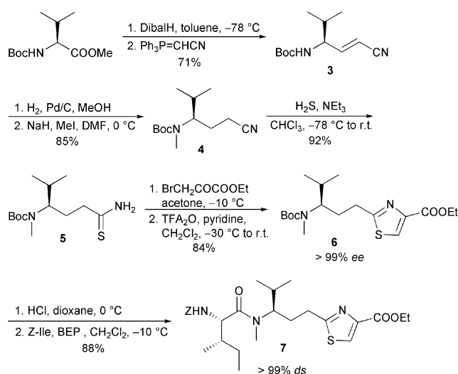
Scheme 1. Synthesis of the Ile-dTuv fragment.
